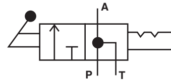
J.I.C. SYMBOL
