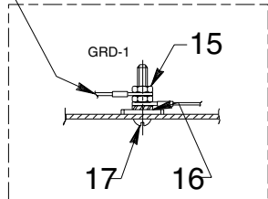
VIEW "A-A"
