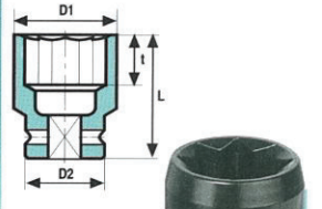
8 POINT IMPACT SOCKETS REGULAR LENGTH
