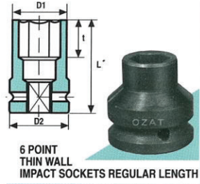
6 POINT THIN WALL IMPACT SOCKETS REGULAR LENGTH
