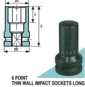
6 POINT THIN WALL IMPACT SOCKETS LONG
