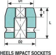
BUD WHEELS IMPACT SOCKETS
